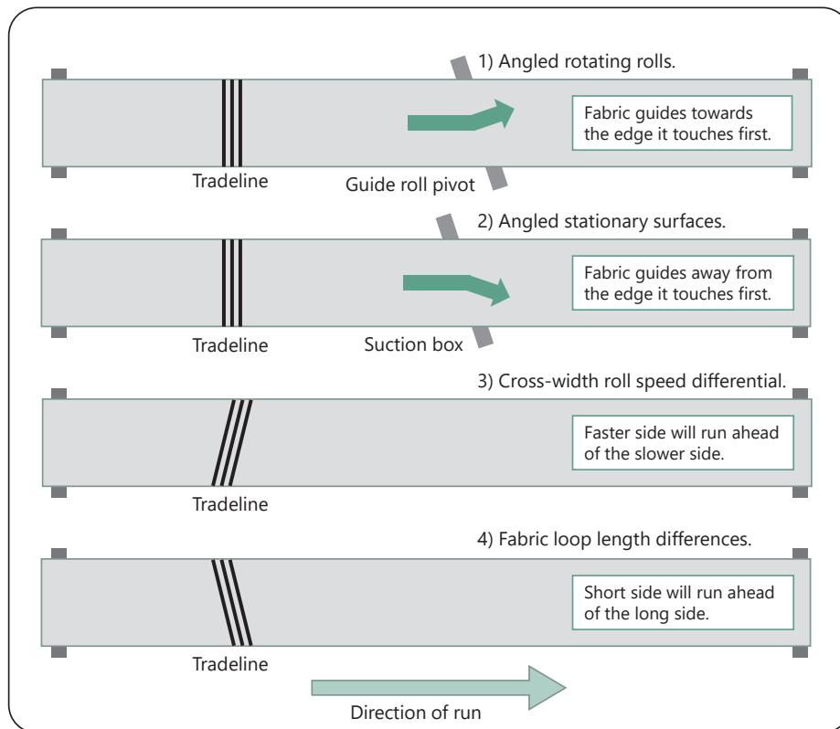
FIGURE 2. Machine factors affecting guiding.
